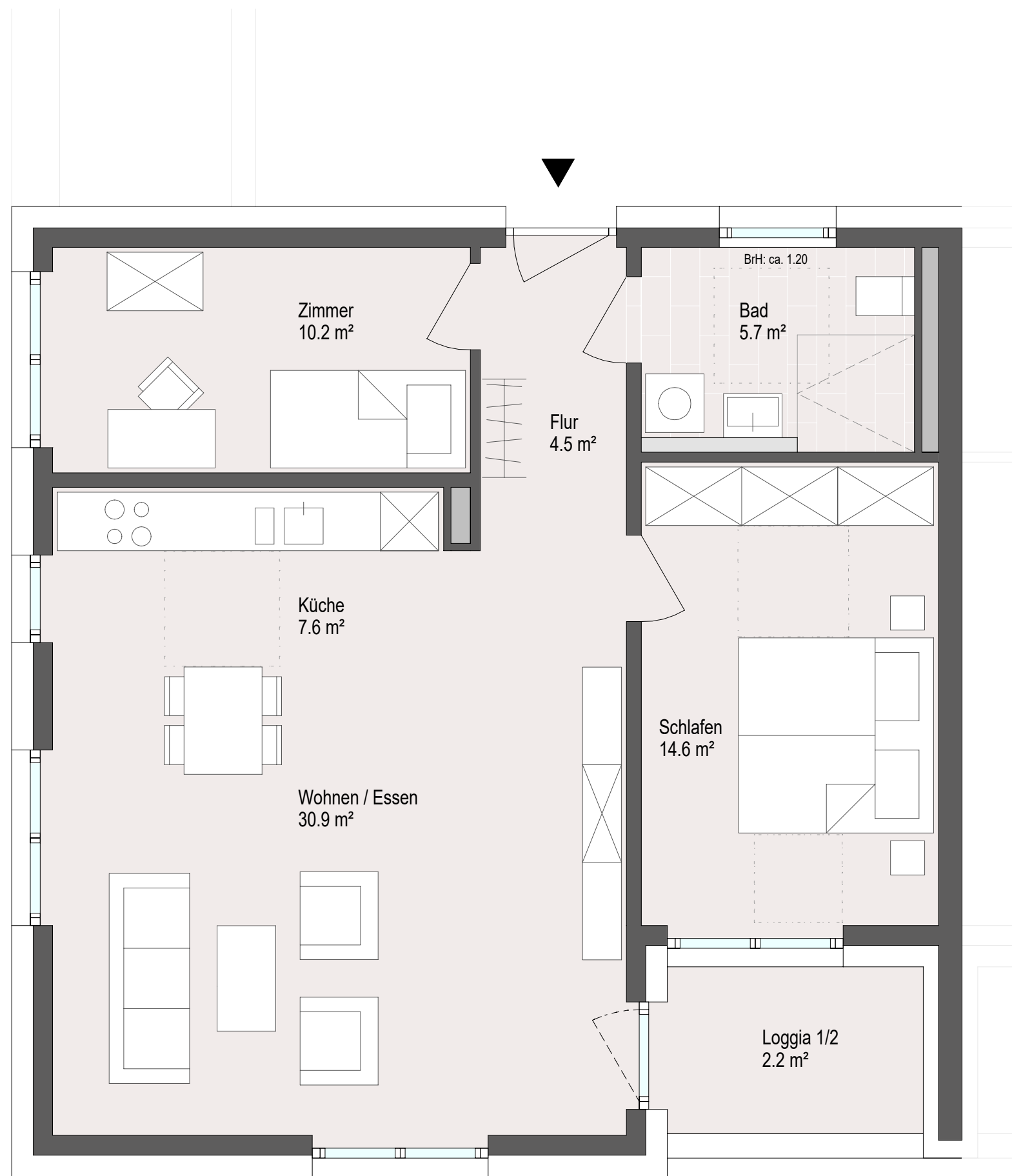
Grundriss 3-Zi-Whg. 75.58m 2
